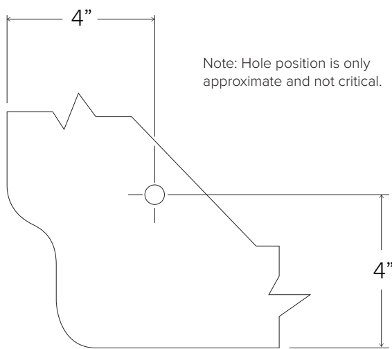
Top view, anchoring flange inside locker
